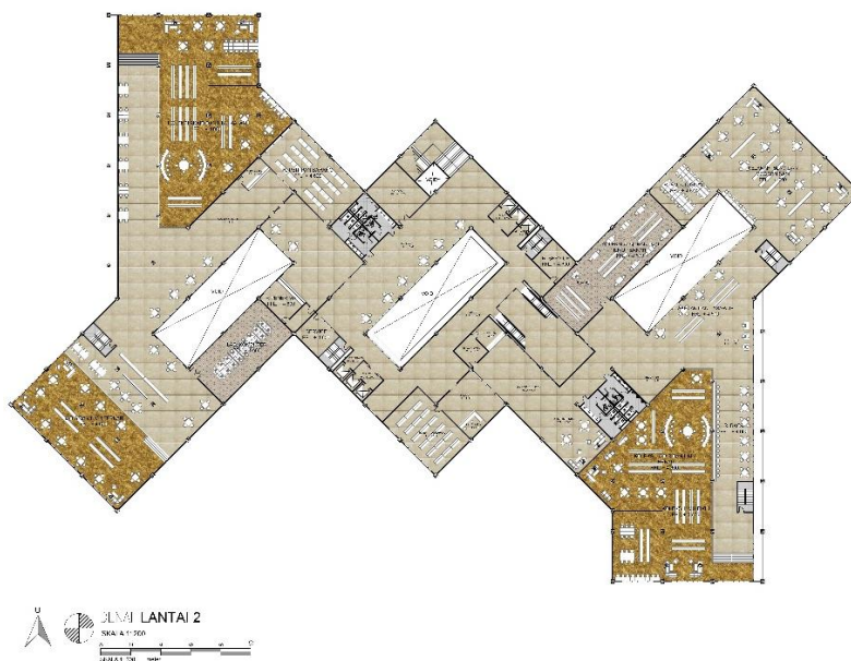
Gambar 1. 6.2.4 "Denah Lantai 2"
