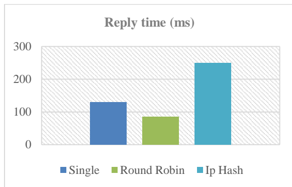
Gambar 10. Reply time
