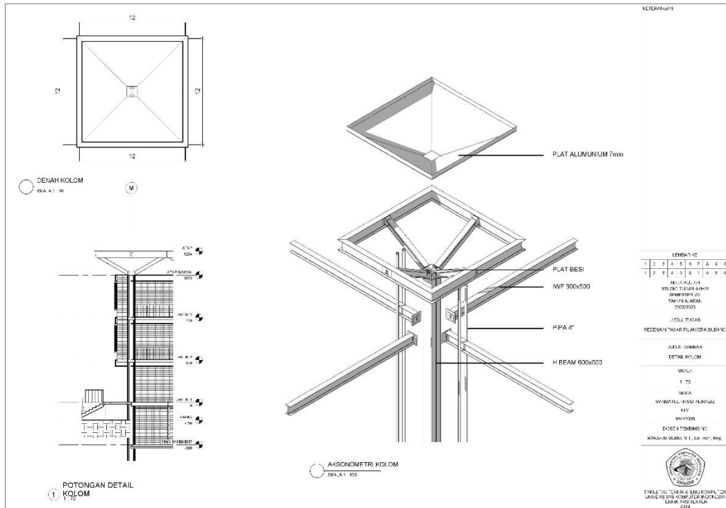
Detail Kolom Atap
