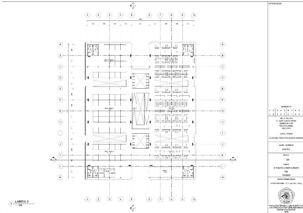
Denah Lantai 3
