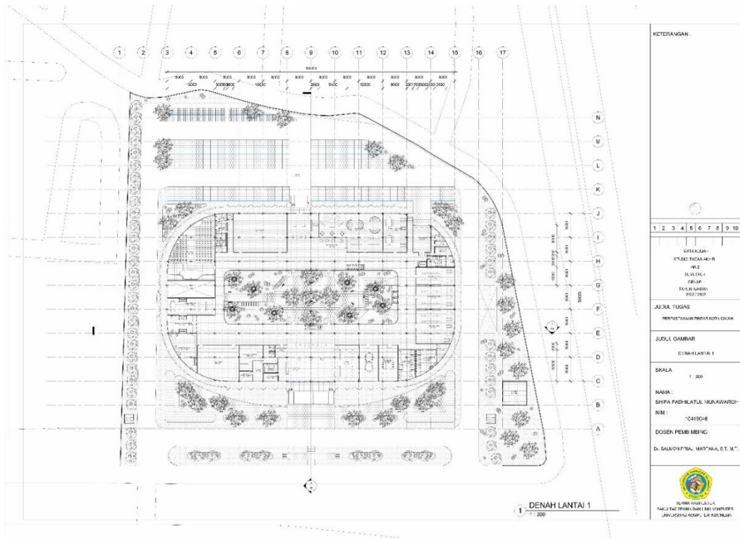
Gambar 6. 3 Denah Lt.1
