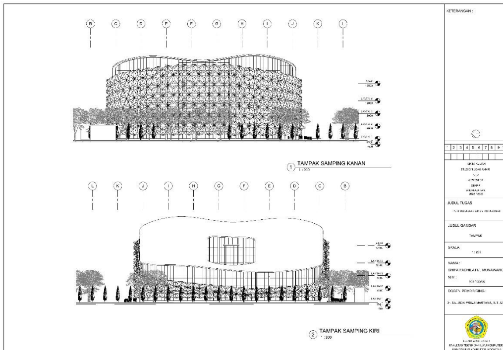
Gambar 6. 8 Tampak Samping
