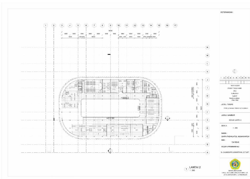
Gambar 6. 4 Denah Lt.2
