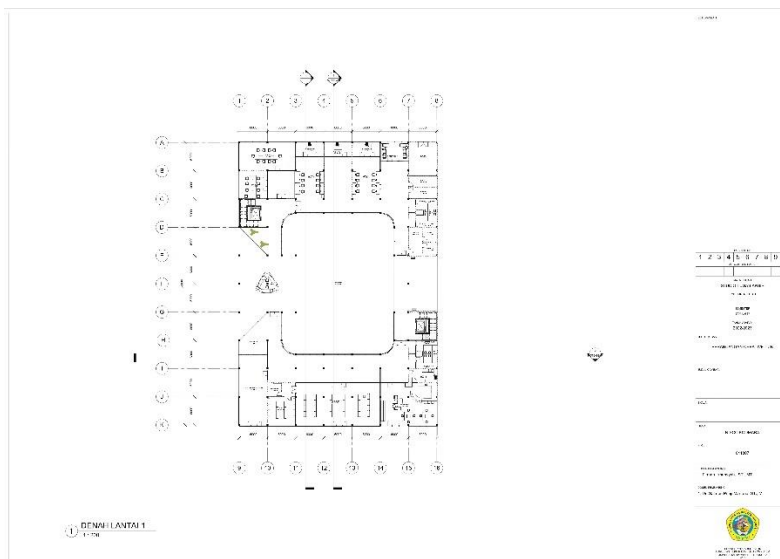
Gambar 6. 5 Denah lantai 1
