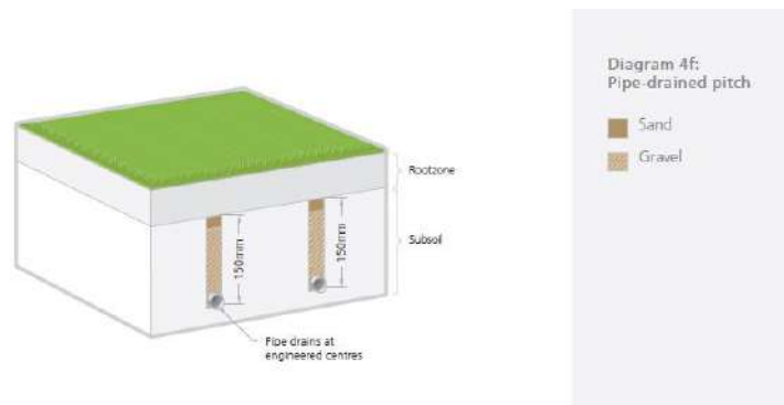
Gambar 2.5 Pipa Drainase Lapangan
