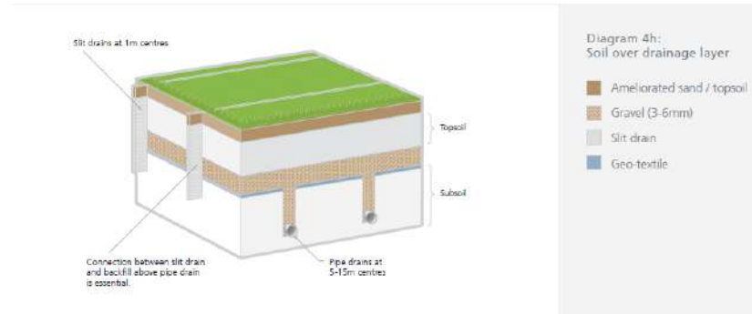
Gambar 2.7 Soil Over Drainage Layer
