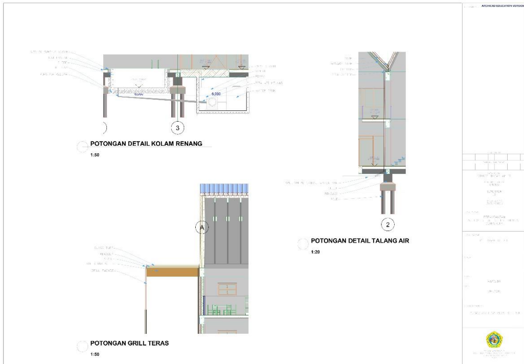
Gambar 6.27 Potongan Detail
