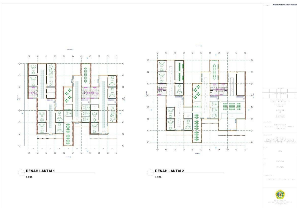
Gambar 6.9 Denah
