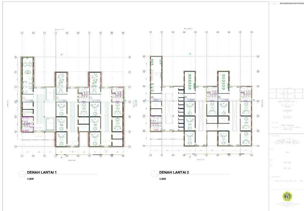
Gambar 6.12 Denah
