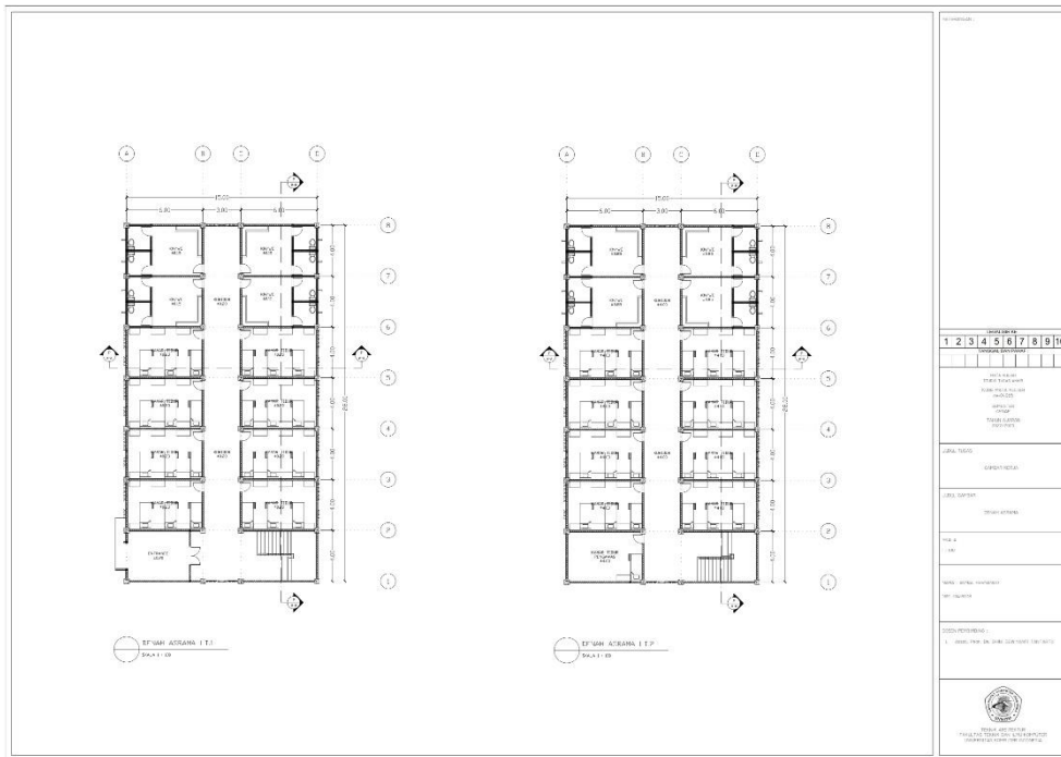
Gambar 6. 9 Denah Asrama
