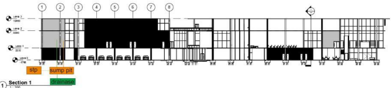
1 Section 1 1:200
