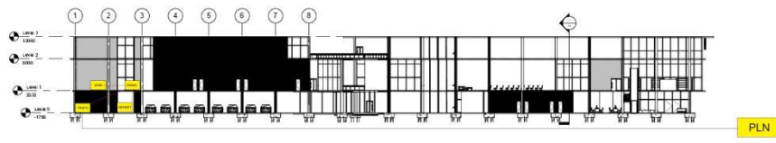
1 Section 1 1:200
