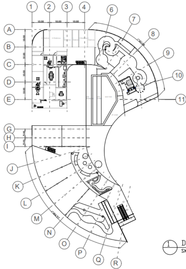
Gambar 6. 3 Denah Lantai 1
