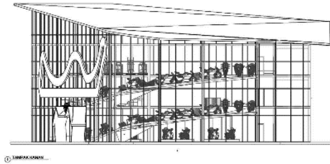
Gambar 6. 16 Tampak Kiri Galeri
