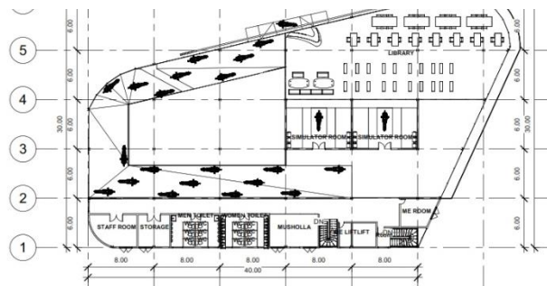
2 DENAH LANTAI 1 1 - 743
