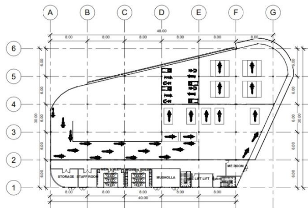
Gambar 6. 3 Denah Galeri Lantai 3
