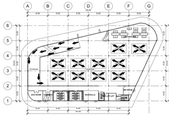
1 DENAH LANTAI DASAR 1 - 742
