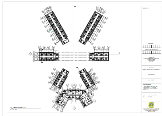
Gambar 6. 5 Denah Lantai 2
