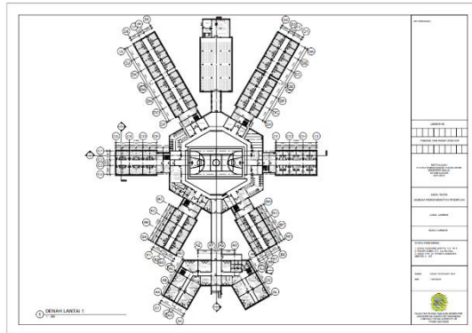
Gambar 6. 4 Denah Lantai 1
