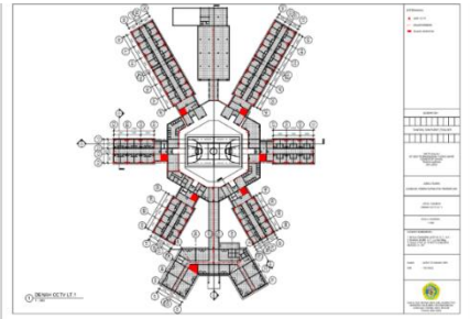
Gambar 6. 16 CCTV
