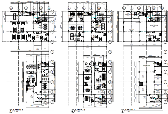
Gambar 45. Denah Coworking 2
