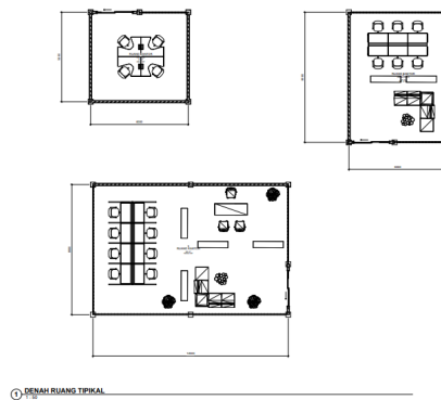
Gambar 47. Denah Tipikal
