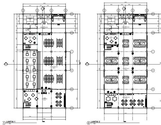
Gambar 43. Denah Coworking 1
