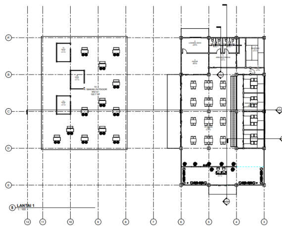
Gambar 41. Denah Cafe
