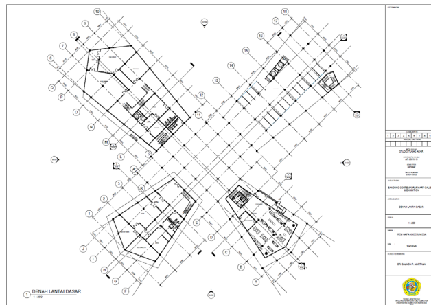
Gambar 6. 3 Denah Lantai Dasar
