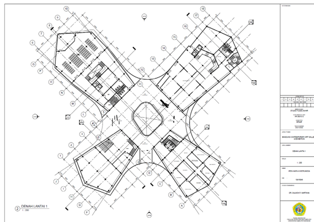
Gambar 6. 4 Denah Lantai 1
