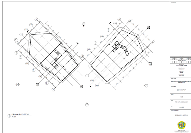
Gambar 6. 7 Denah Lantai Atap
