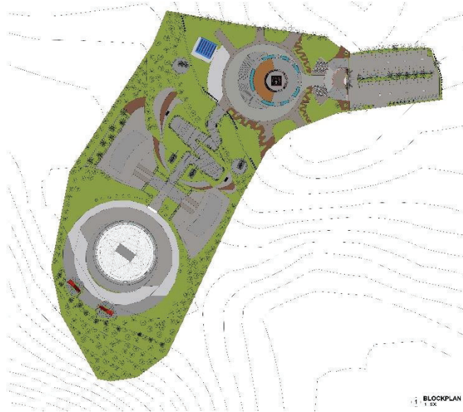
Gambar 6. 1 Blockplan
