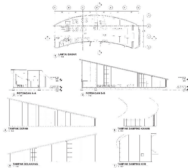
Gambar 6. 13 Denah, Tampak, Potongan Cafe & Souvenir Center
