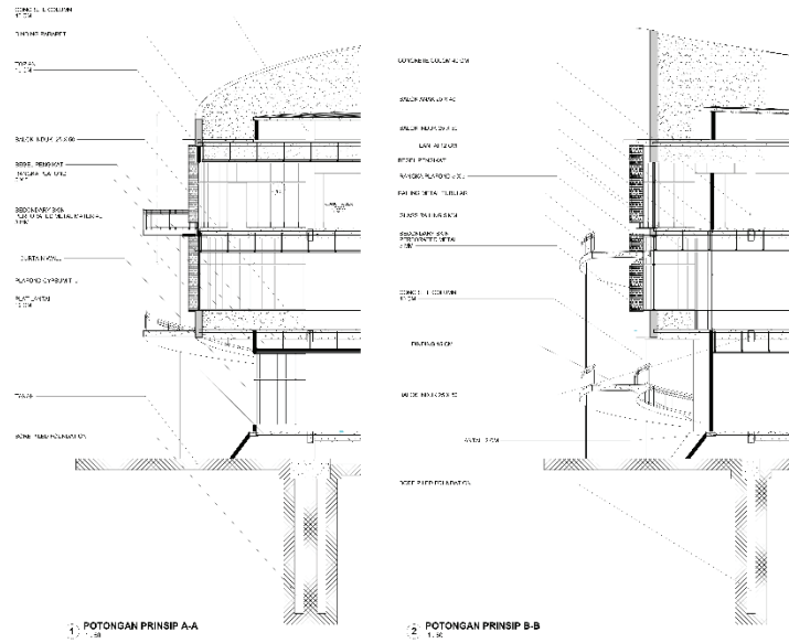
Gambar 6. 9 Potongan Prinsip Museum
