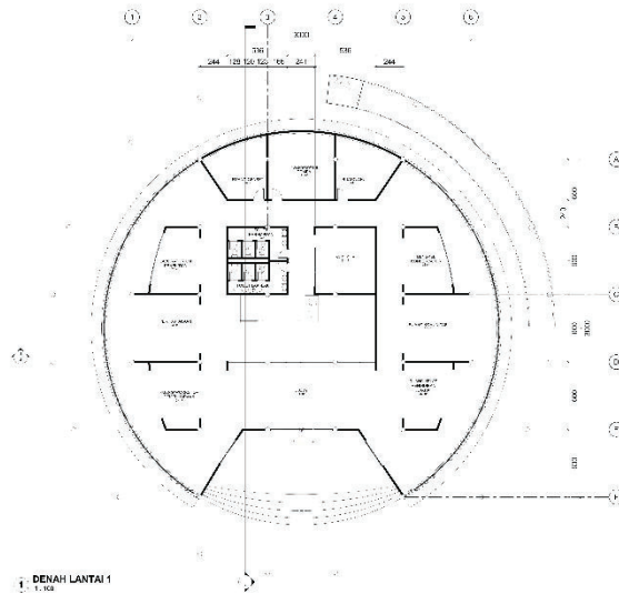
Gambar 6. 4 Denah Museum Lantai 1
