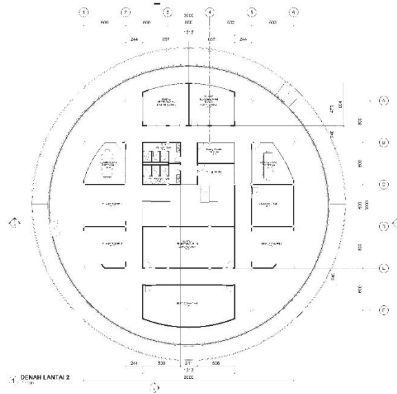
Gambar 6. 5 Denah Museum Lantai 2
