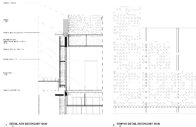
Gambar 6. 21 Detail Façade
