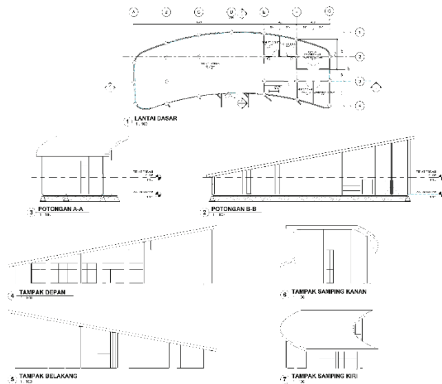
Gambar 6. 12 Denah, Potongan, Tampak Sanggar Seni
