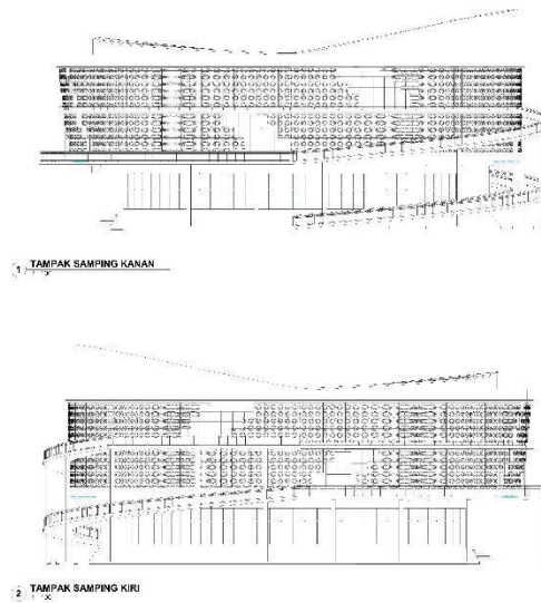
Gambar 6. 11 Tampak Samping Museum
