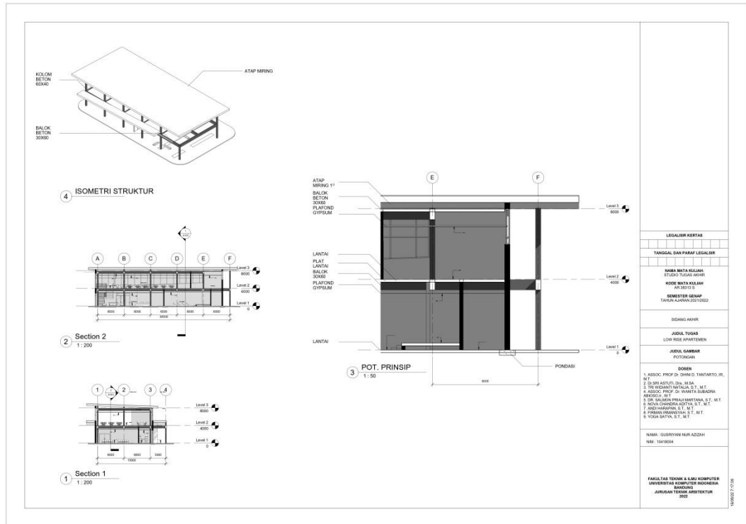
Gambar 6. 17 Potongan, Isometri Struktur & Pot. Prinsip Main Lobby
