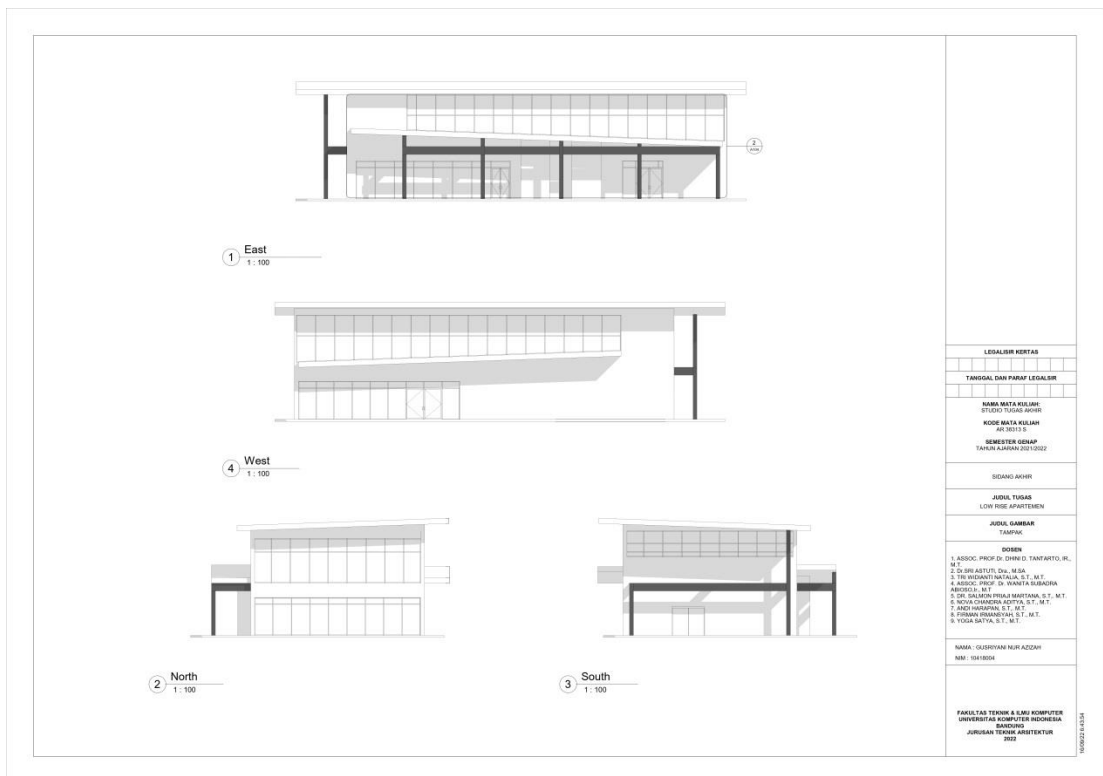
Gambar 6. 16 Tampak Main Lobby
