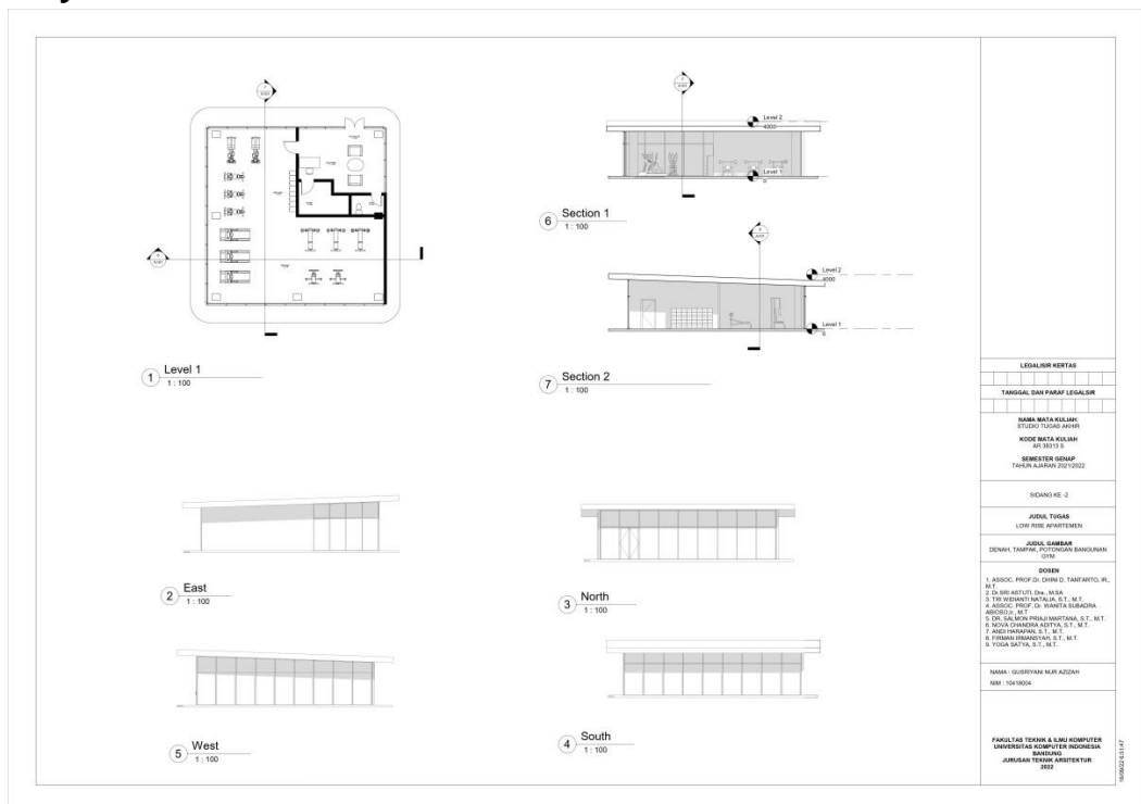
Gambar 6. 18 Denah, Tampak & Potongan Gym Indoor
