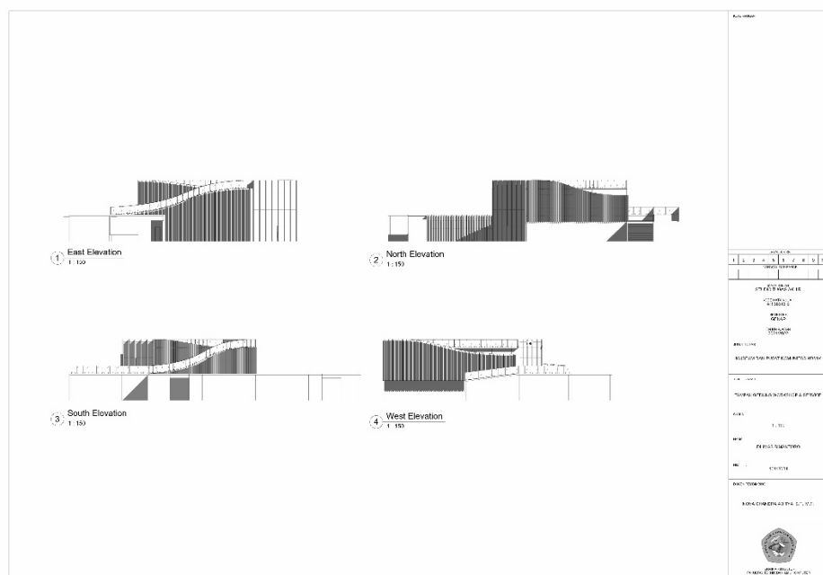
Gambar 6. 16 Tampak Workshop & Service
