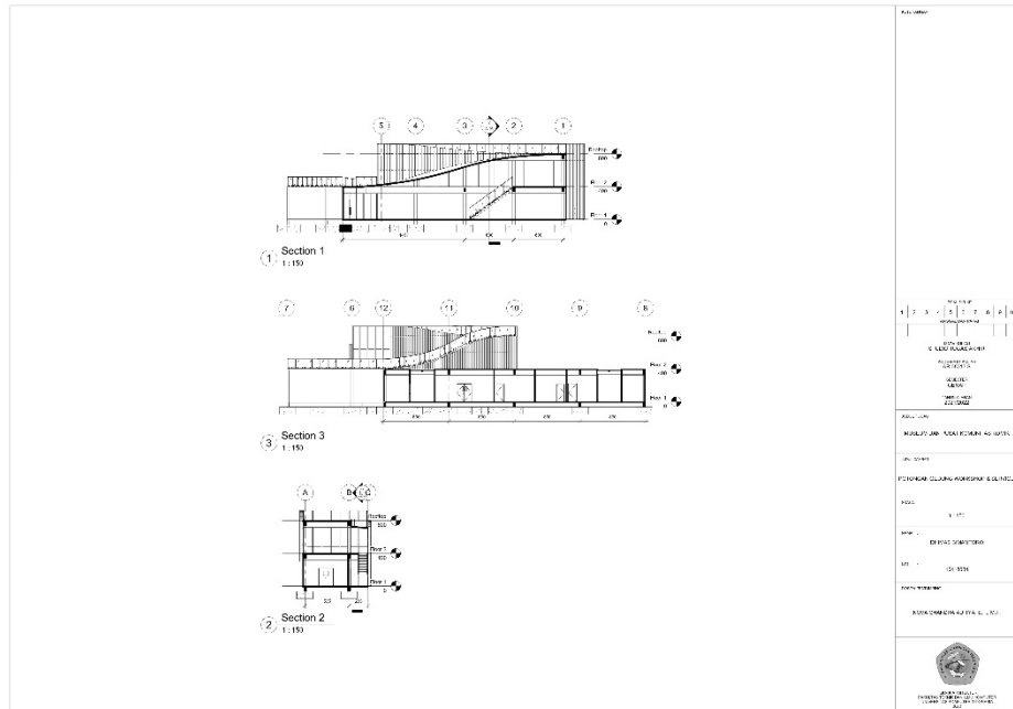
Gambar 6. 17 Potongan Workshop & Service
