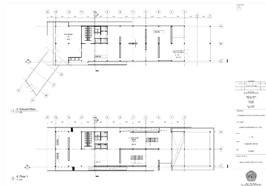
Gambar 6. 6 Denah Museum (Ground Floor & 1st Floor)
