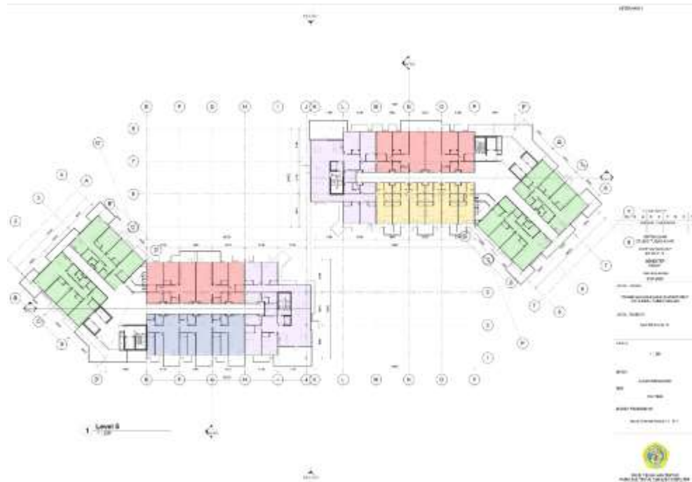
Gambar VI.6 Denah Lt. 5,9,14,18
