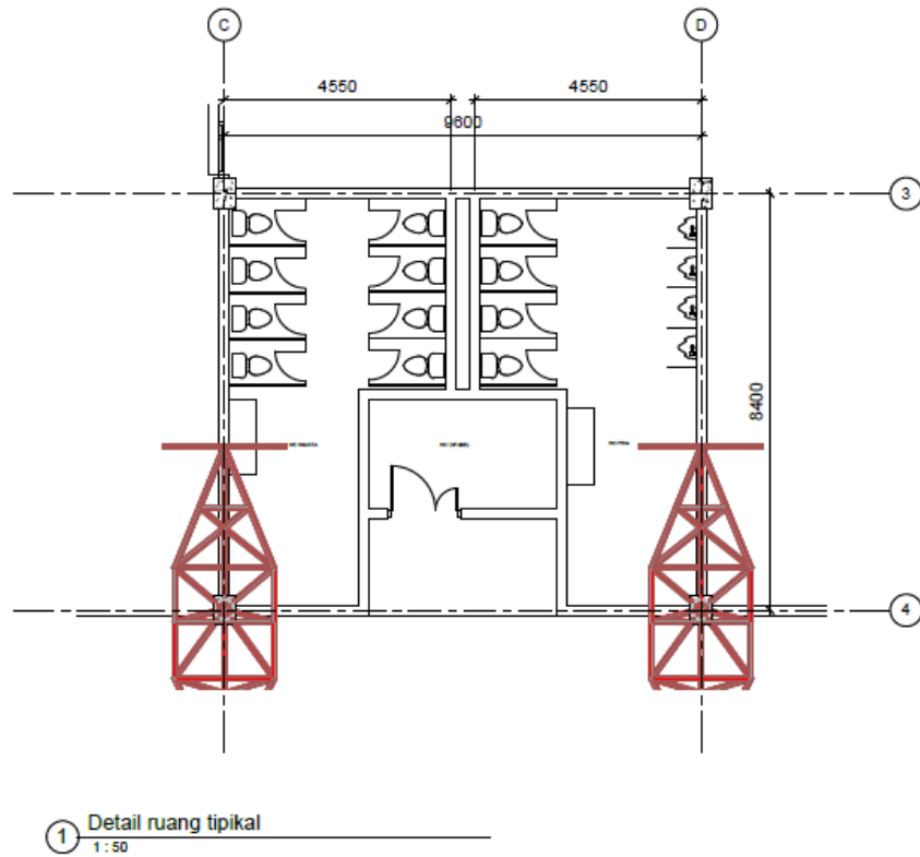
Gambar 6. 5 Denah ruang tipikal
