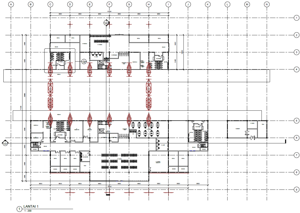
Gambar 6. 3 Denah lantai 1
