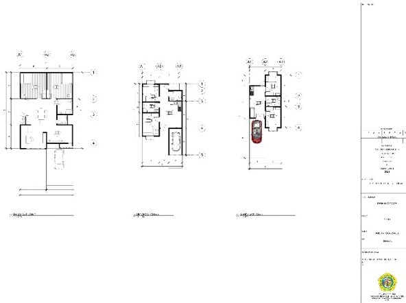
Gambar 6. 8 Denah Cottage
