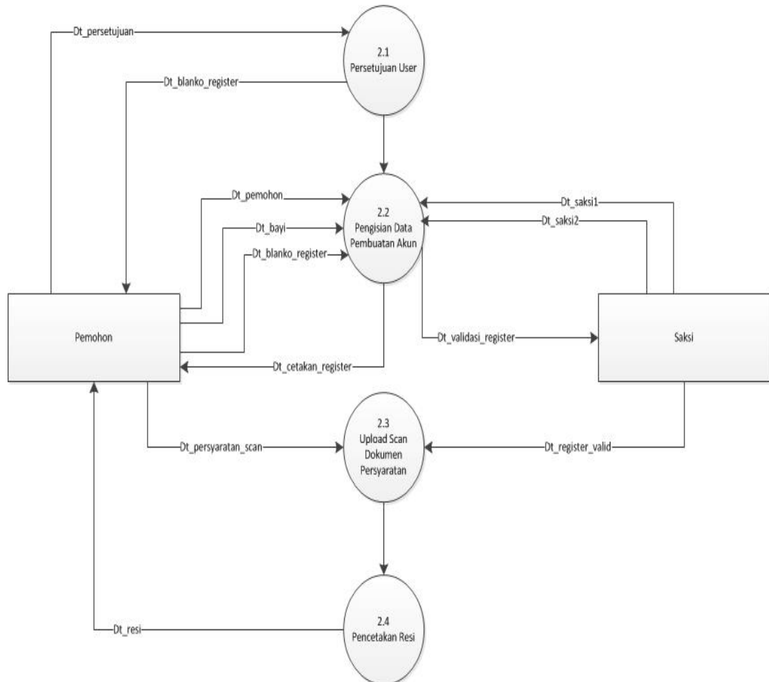
Gambar 4.9 : DFD Level 1 Proses 2 Pengisian Form
