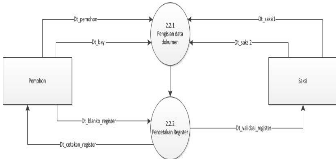
Gambar 4.12 DFD Level 2 Proses 2.2 Pengisian Data
