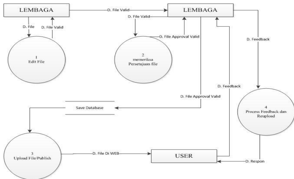
Gambar 4. 3. DFD Level 0
