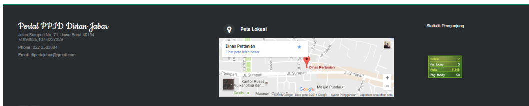
Gambar 4. 6. Submenu UU
