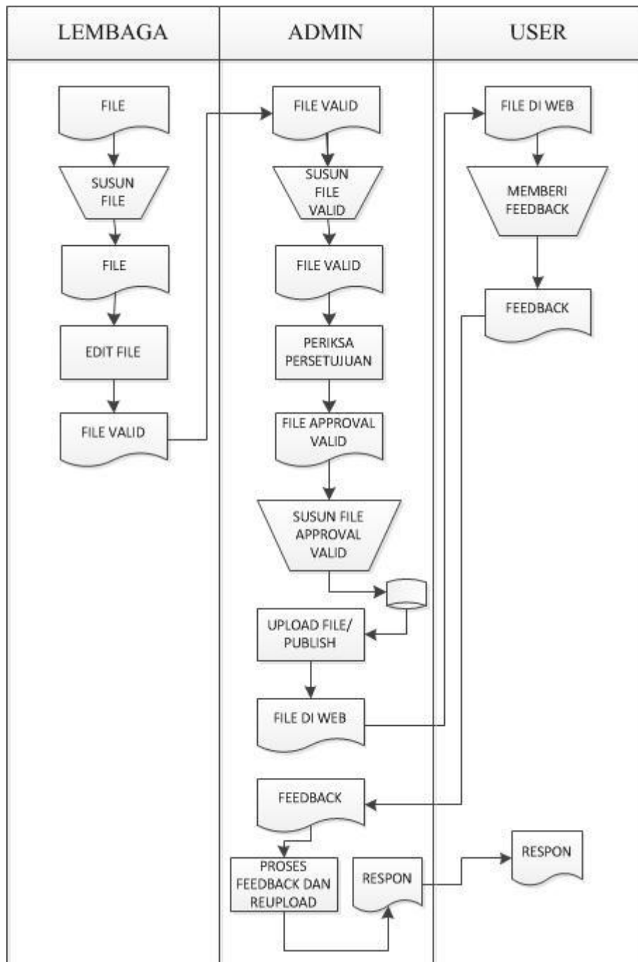
Gambar 4. 1. Flowmap
