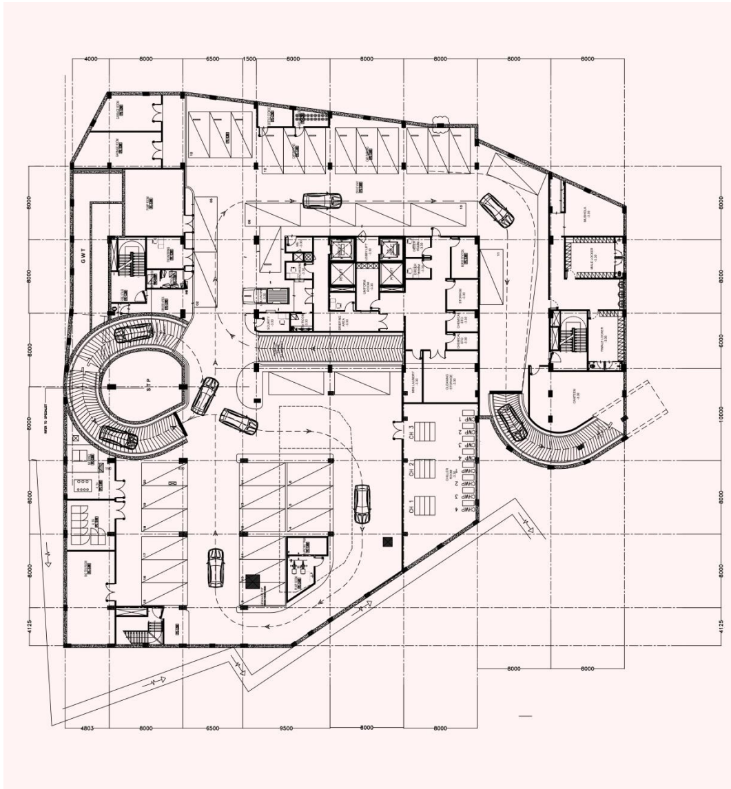
Gambar 3 5 Blocking Basement
