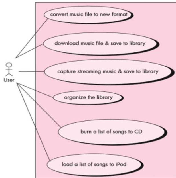
Gambar 2. 4 Contoh Usecase Diagram
