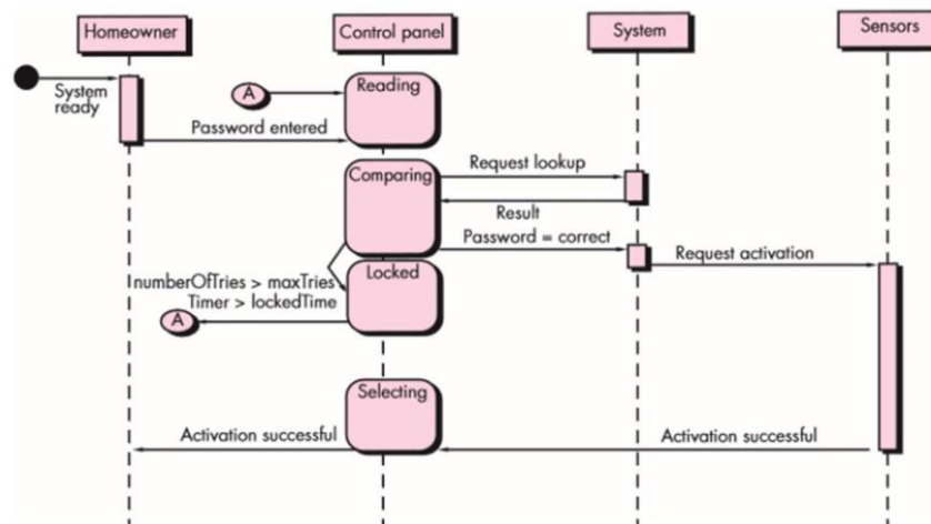
Gambar 2. 6 Contoh Sequence Diagram
