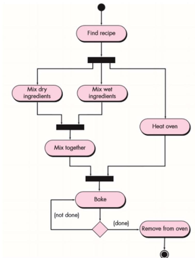
Gambar 2. 5 Contoh Activity Diagram
