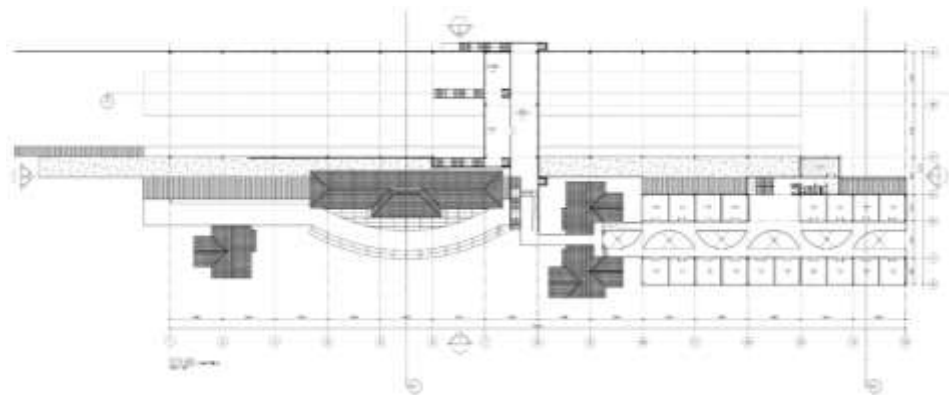
Gambar 6.4 Denah Lantai 2
