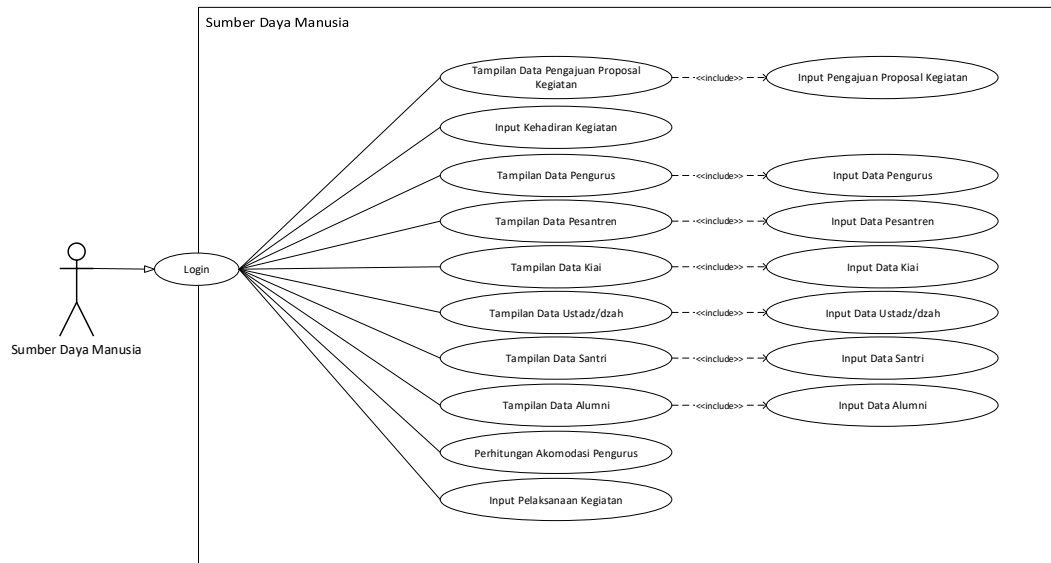
Gambar 4.6 Use Case Diagram Package Sumber Daya Manusia
