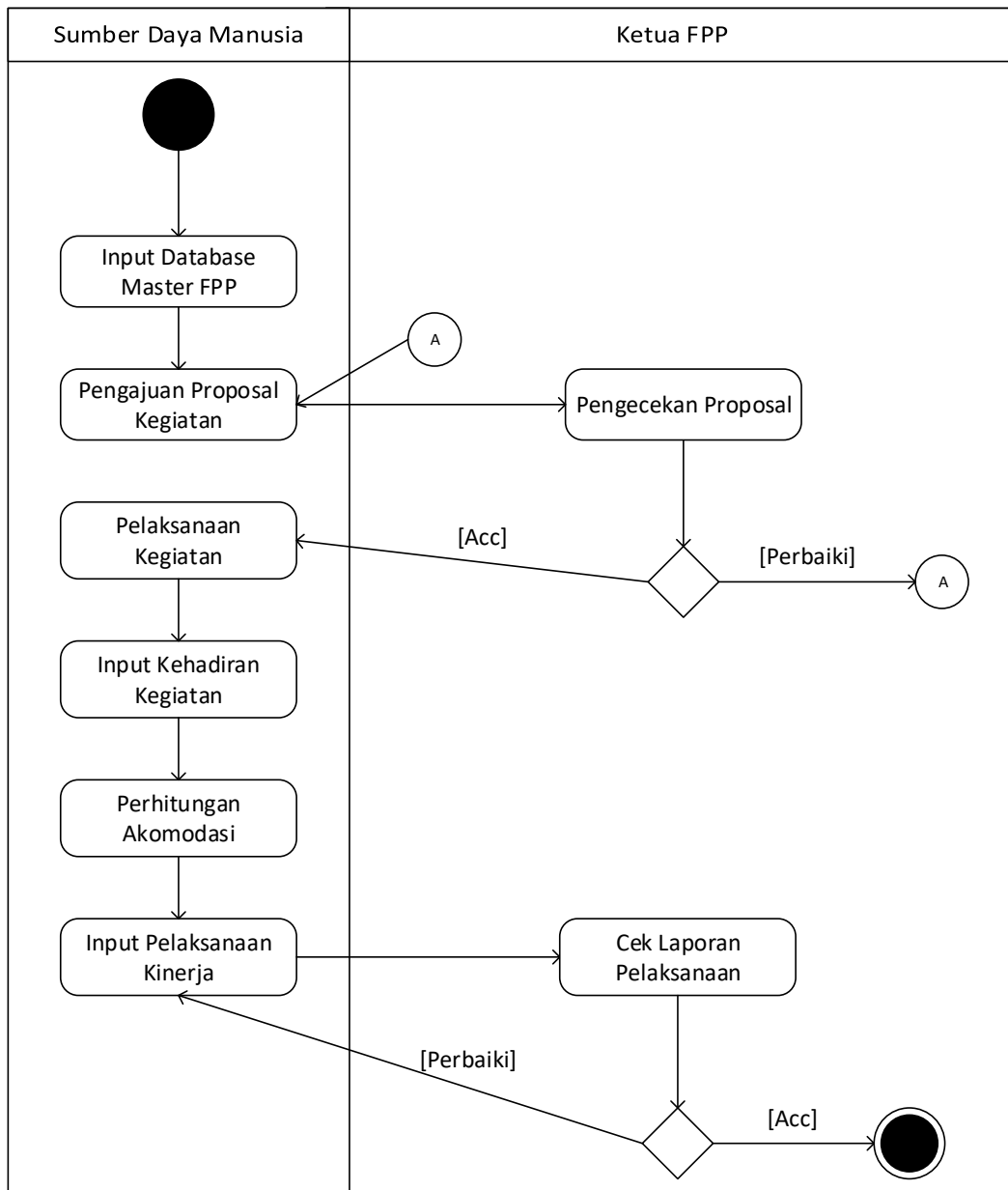
Gambar 4.10 Sub Activity Sumber Daya Manusia
