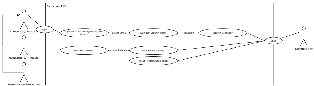
Gambar 4.4 Use Case Package Diagram Sekretaris
