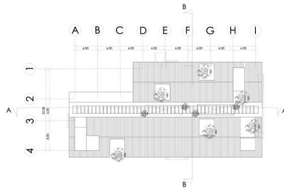
ROOF LEVEL PLAN HUNIAN RT 03
