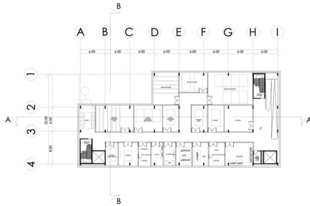
SEMI BASEMENT LEVEL PLAN HUNIAN RT 03
