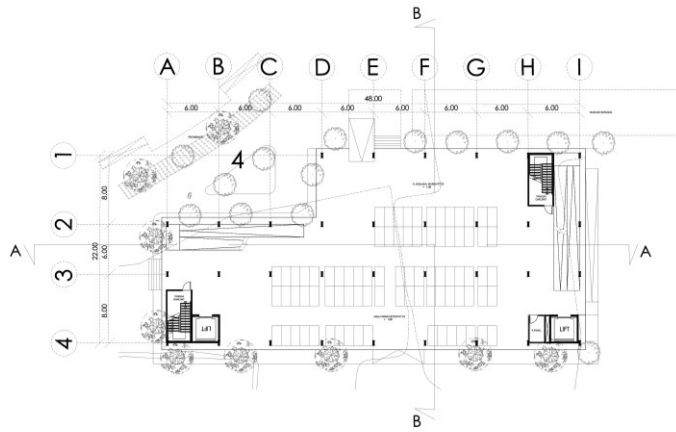
GROUND LEVEL PLAN HUNIAN RT 03
