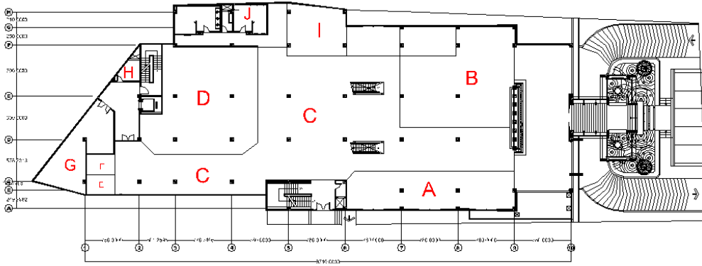
GROUND FLOOR PLAN SC: 1/150
