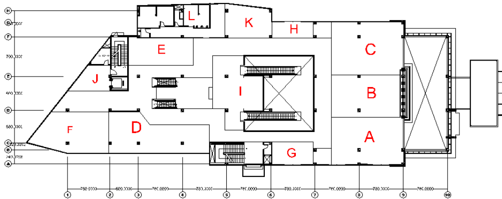
1ST FLOOR PLAN SC: 1/150
