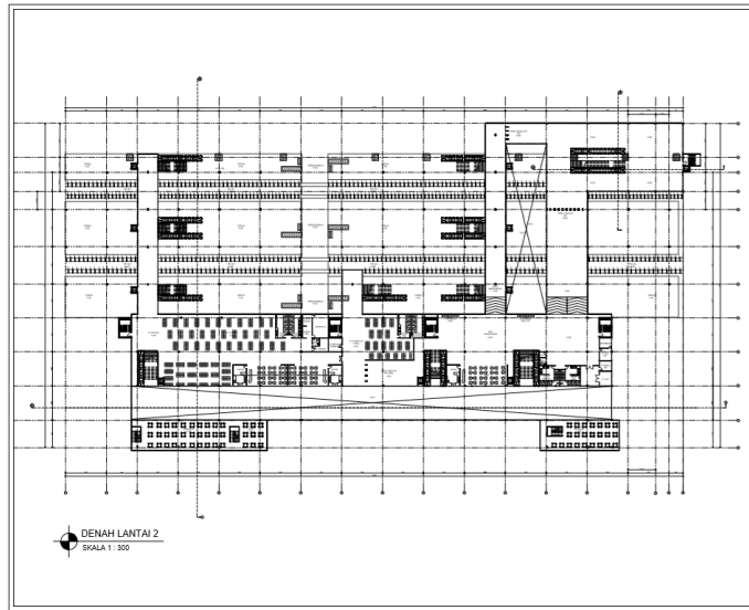
Gambar 6.3 Denah Lantai 2
