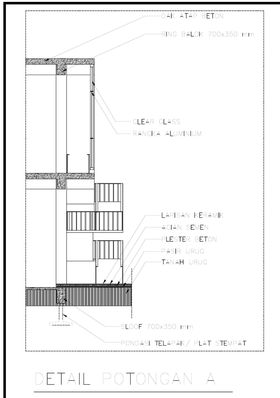
Gambar 6.13. Detail 1
