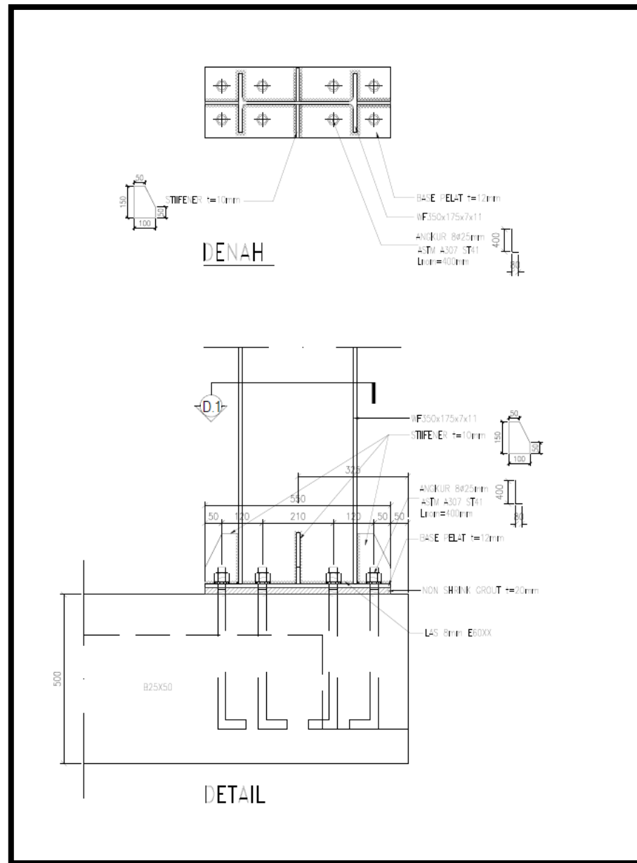
Gambar 6.14. Detail 2
