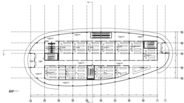
Gambar 6.5 Denah Lantai 1 Retail Sumber : Data Pribadi
