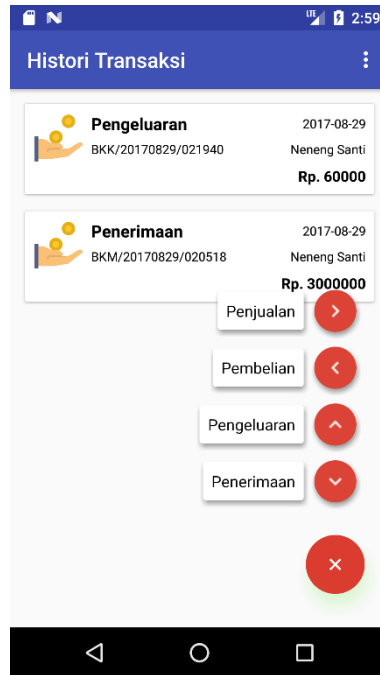
Gambar 4.35 Tampilan TransaksiActivity
