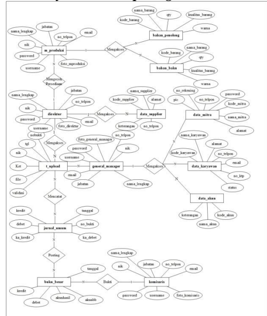
Gambar 15 Entity Relationship Diagram
