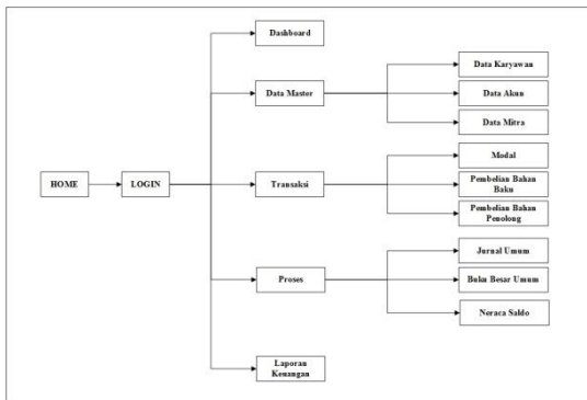
Gambar 19 Struktur Menu General Manager
