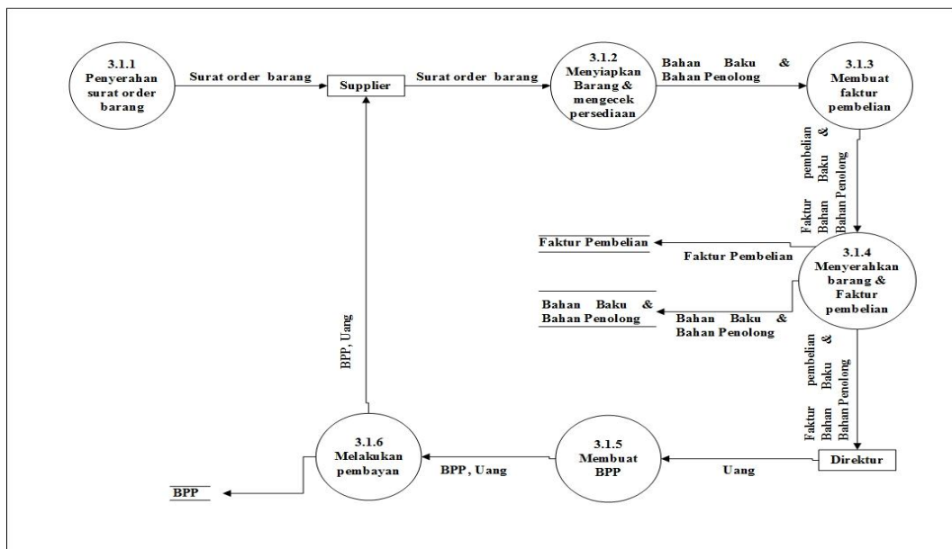
Gambar 4.7 Data Flow Diagram Level 2 Proses 1 Usulan
