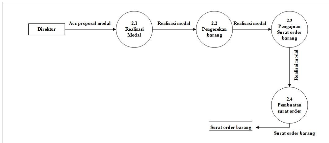
Gambar 4.5 Data Flow Diagram Level 1 Proses 2 Usulan
