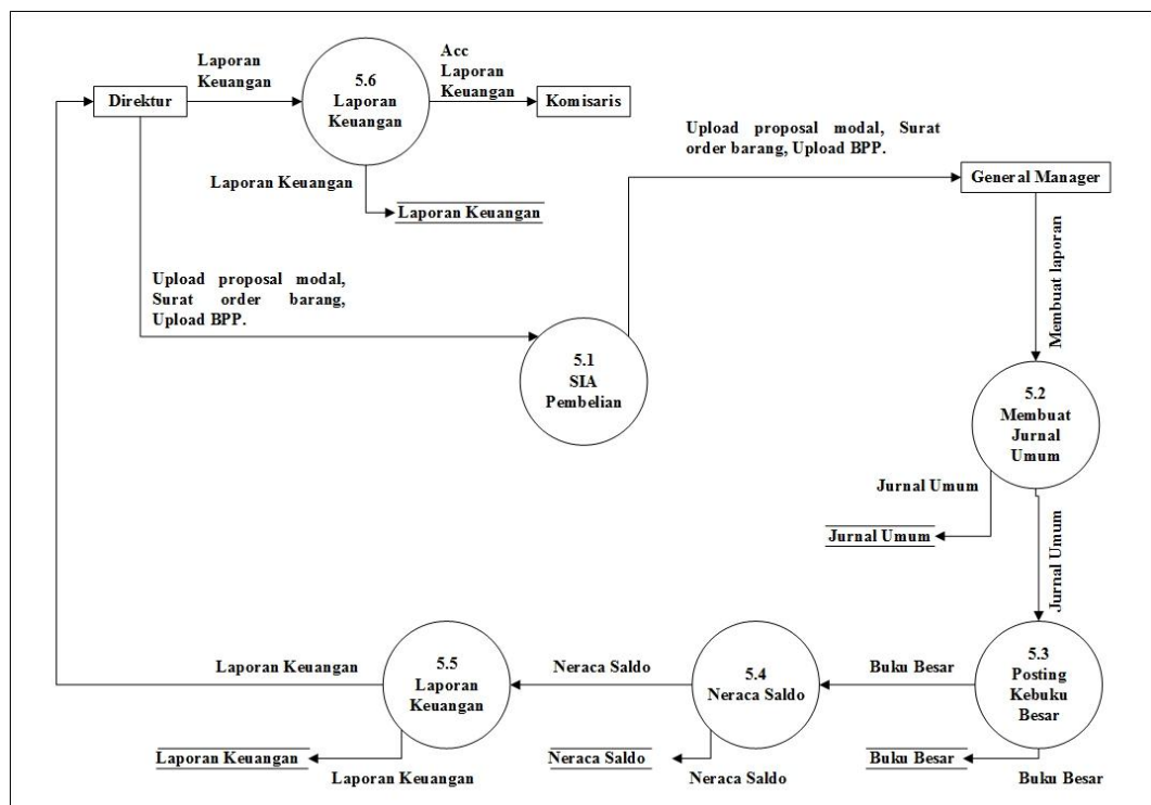
Gambar 4.9 Data Flow Diagram Level 1 Proses 5 Usulan
