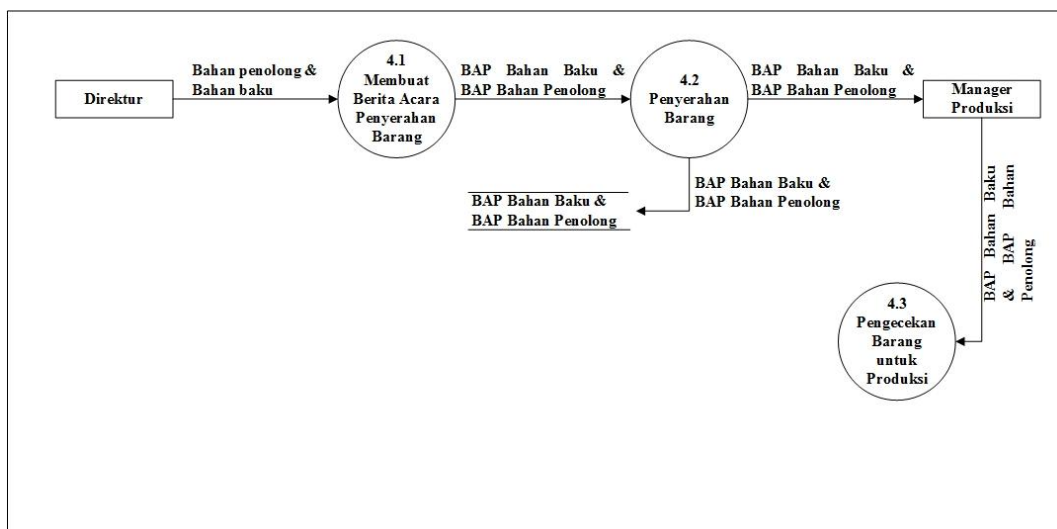
Gambar 4.8 Data Flow Diagram Level 1 Proses 4 Usulan
