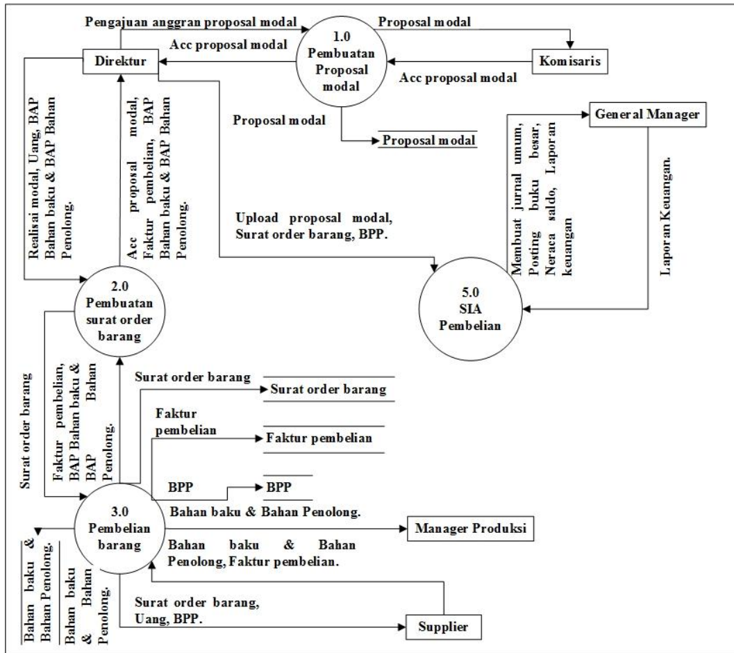
Gambar 4.2 Data Flow Diagram Level 0 Usulan
