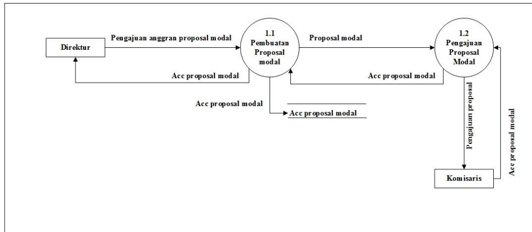
Gambar 4.4 Data Flow Diagram Level 1 Proses 1 Usulan
