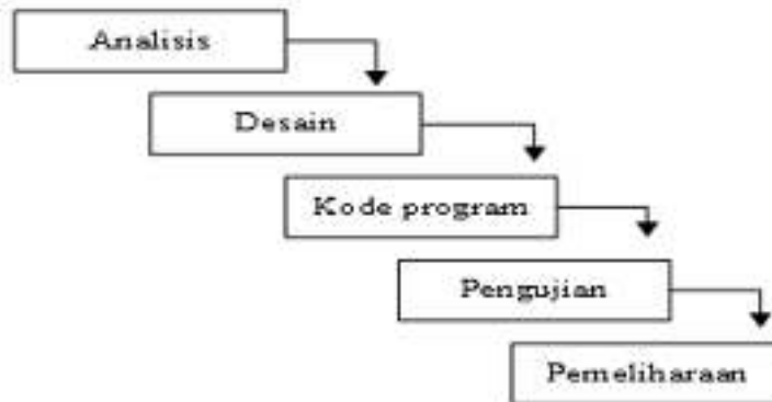
Gambar 1 Model Waterfall
