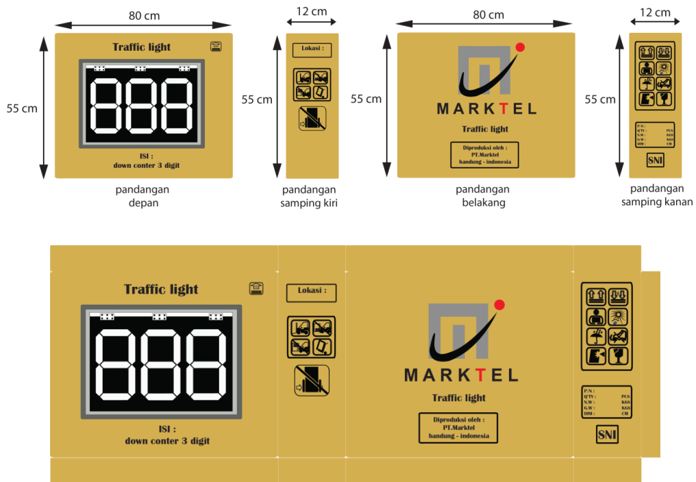
Gambar IV.27 Visual Kemasan Traffic Light,down conter 3 digit
