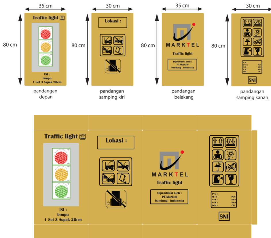
Gambar IV.22 Visual Kemasan Traffic Light, lampu 1 set 3 aspek 20 cm
