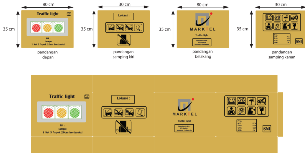
Gambar IV.24 Visual Kemasan Traffic Light,lampu 1 set 3 aspek 20 cm (horizontal)
