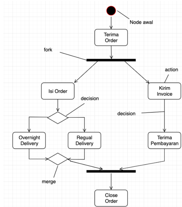
Gambar 2. 15 Activity Diagram [10]
