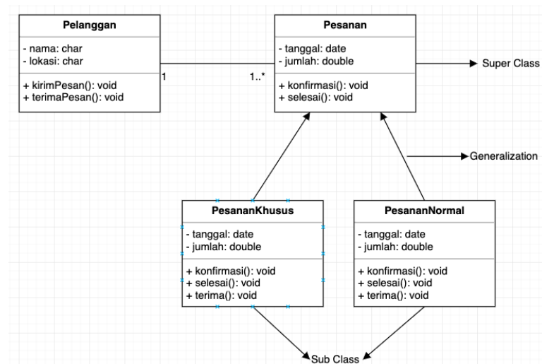
Gambar 2. 14 Class Diagram [10]
