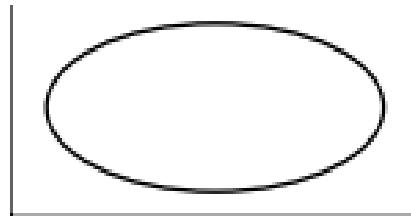
Gambar 2. 12 Use Case [10]
