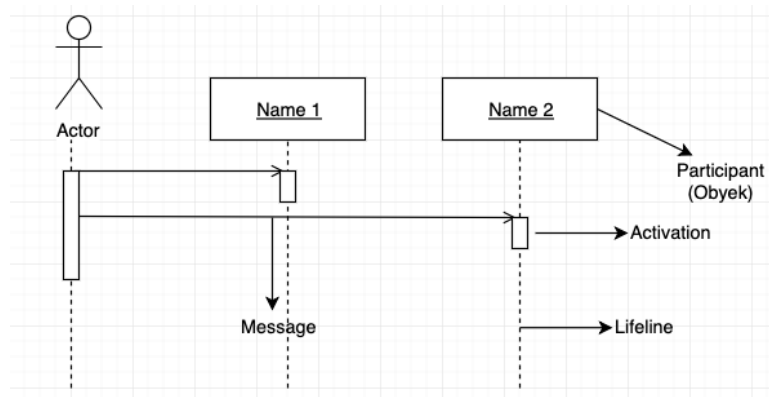
Gambar 2. 16 Sequence Diagram [10]
