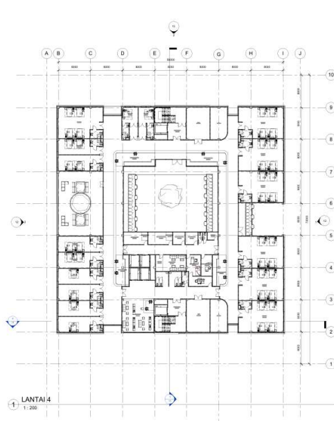
Gambar 6.6 Denah Lantai 4
