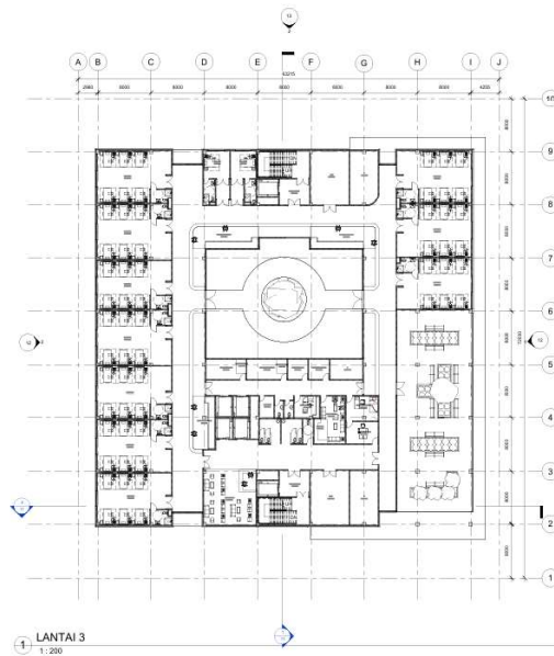
Gambar 6.5 Denah Lantai 3
