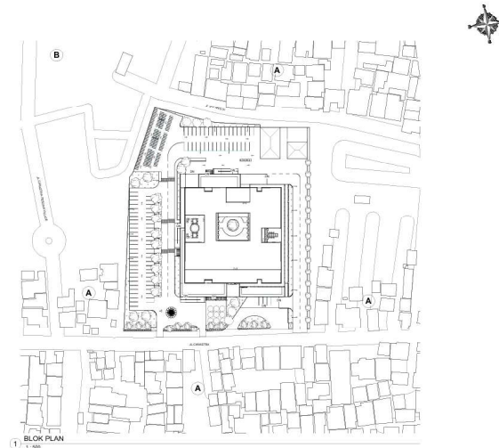
Gambar 6.1 Blokplan
