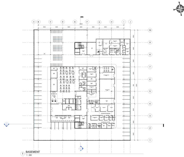
Gambar 6.7 Denah Basemen
