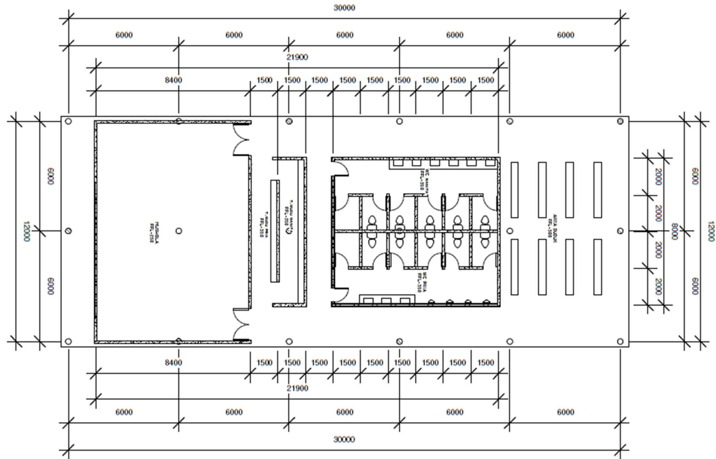
Gambar 6. 6 Denah Gd. Istirahat
