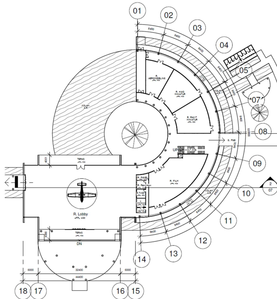
Gambar 6. 3 Denah Lt.1 Gd. Penerima
