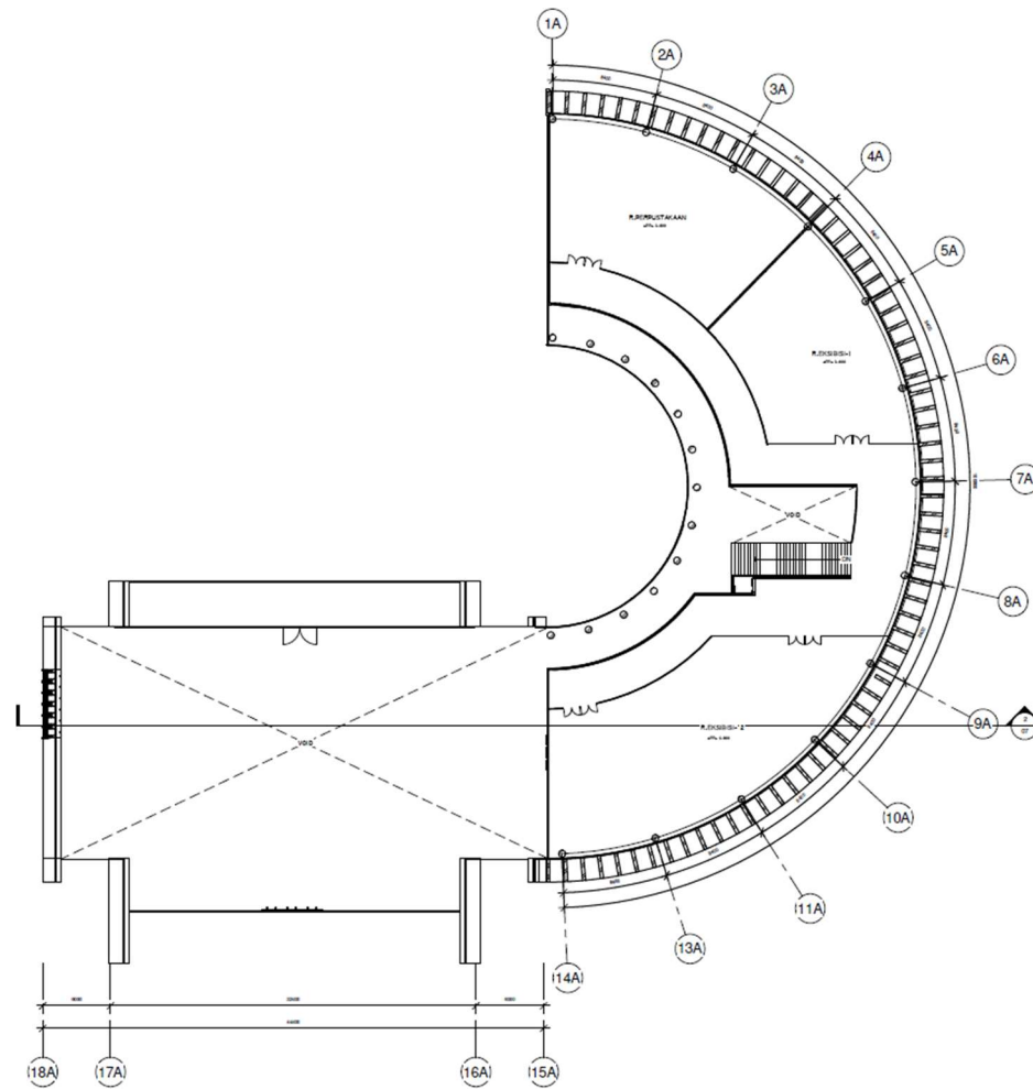
Gambar 6. 7 Denah Lt.2 Gd. Penerima
