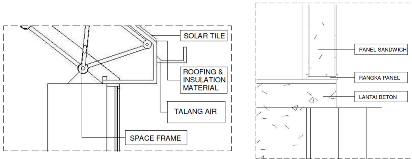
Gambar 6. 12 Potongan Detail
