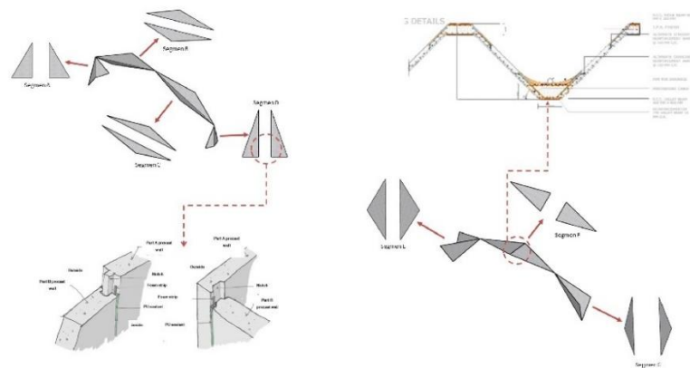
Gambar 6. 14 Folded plate system (Sumber: Dokumen pribadi)
