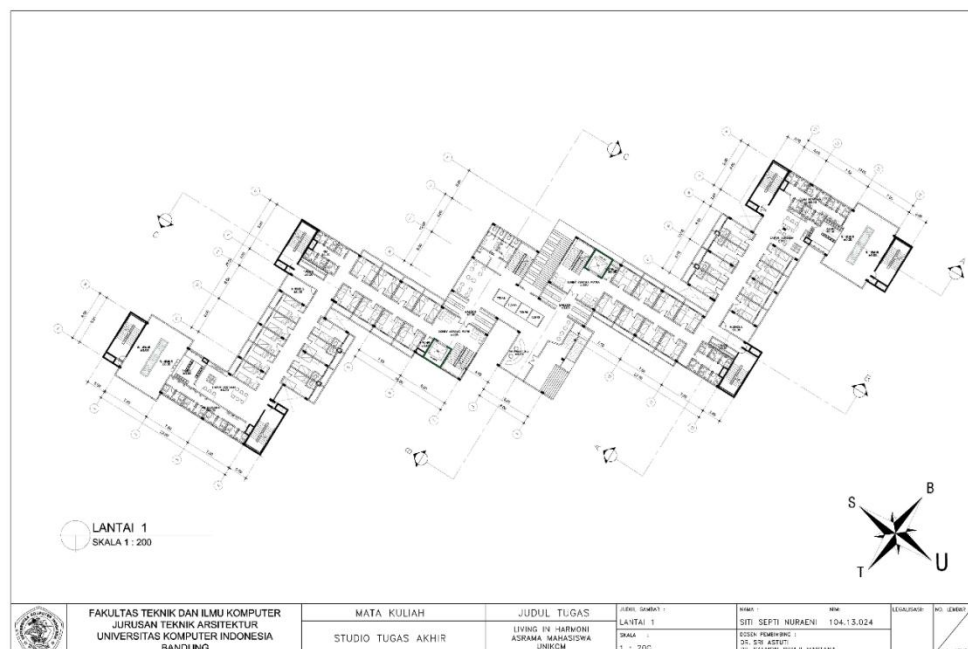
Gambar 6.4 Denah Lantai 1
