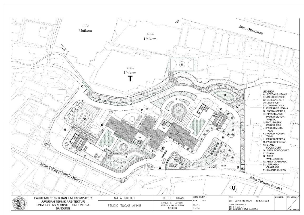
Gambar 6.1 Siteplan
