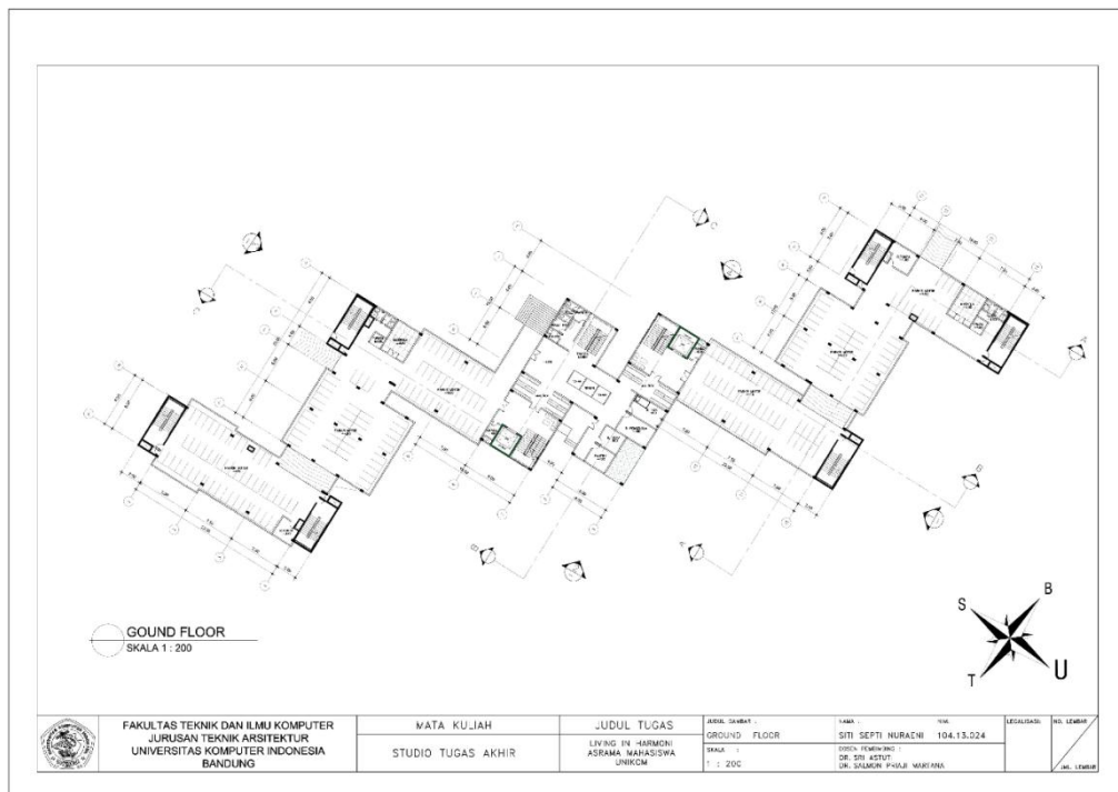
Gambar 6.3 Ground Floor
