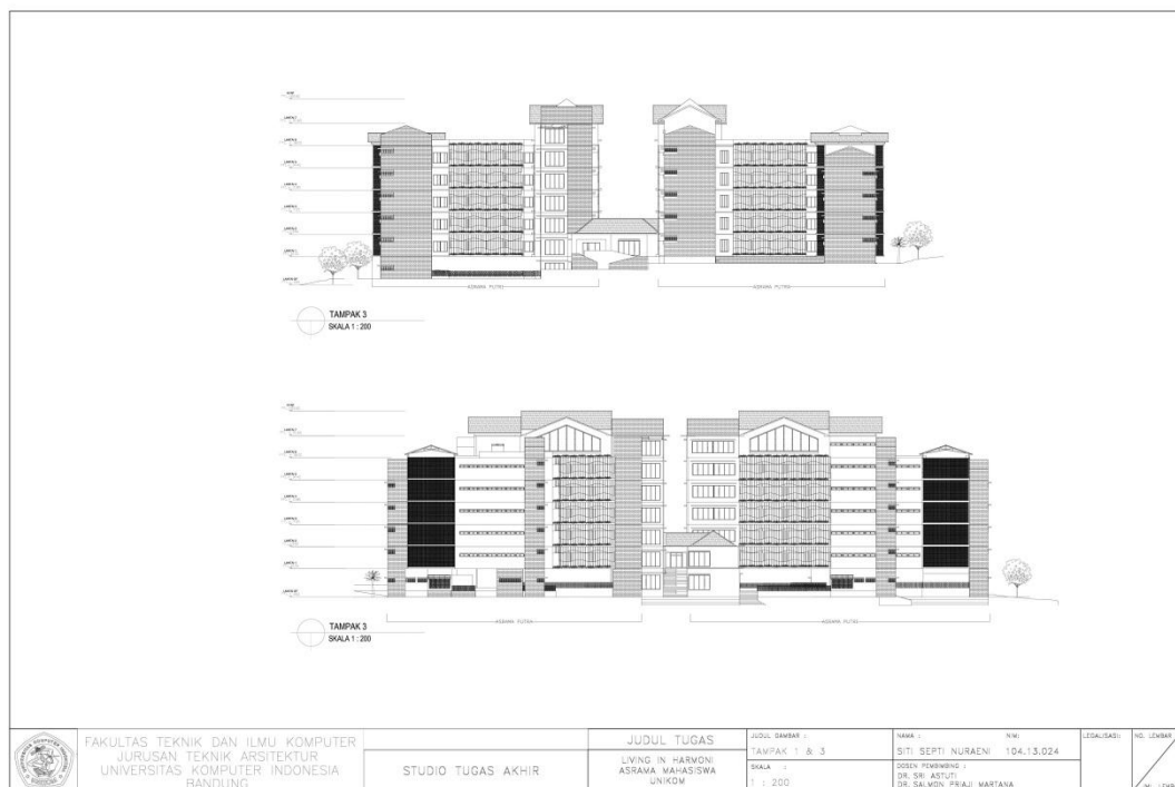
Gambar 6.13 Tampak 1-3
