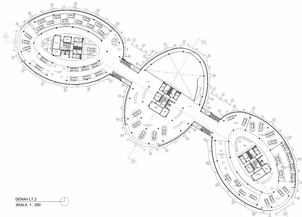
Gambar 6.4. Denah Lt.2 Toyota Automobile Museum Center
